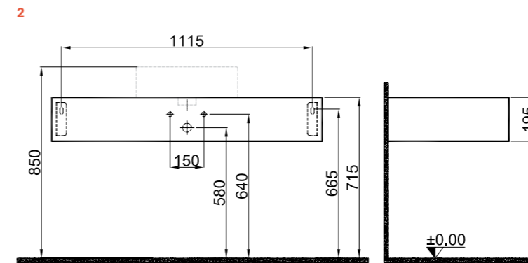
K-2 160 Sinterflex Counter Front and Side View
