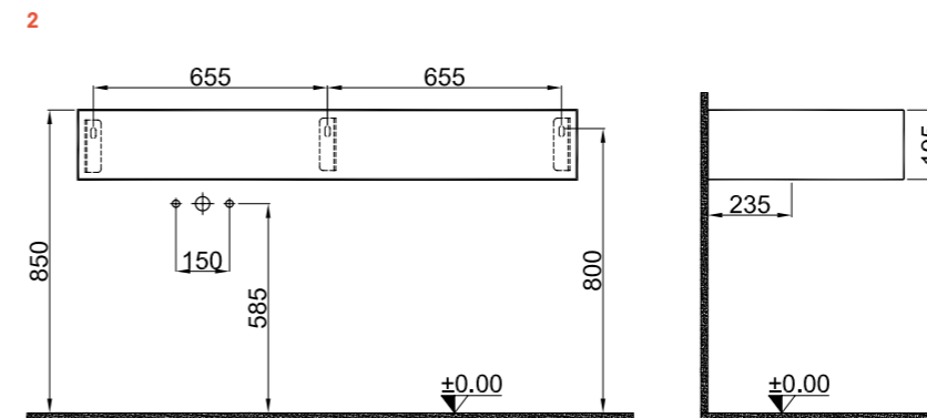
K-1 140 Sinterflex Lavabolu Tezgah Ön ve Yan Görünüş / K-1 140 Sinterflex Counter with Washbasin Front and Side View
