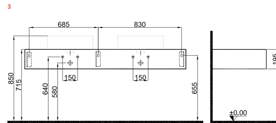
K-2 160 Sinterflex Counter Front and Side View
