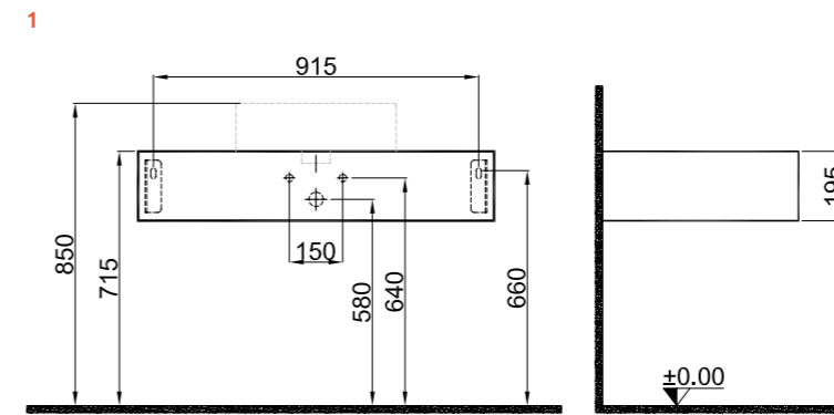
K-2 100 Sinterflex Counter Front and Side View
